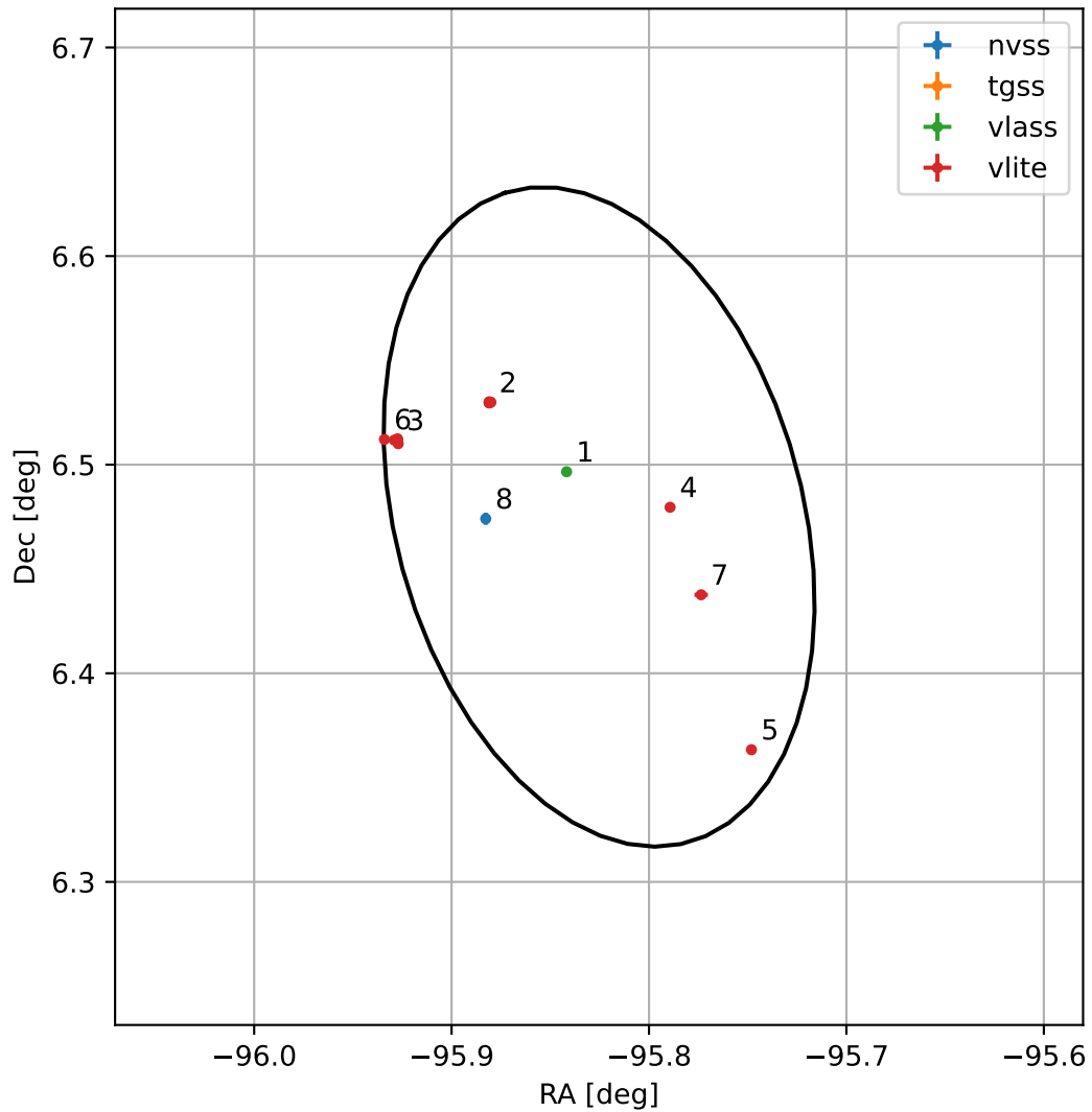
4FGL J1736.6+0628
