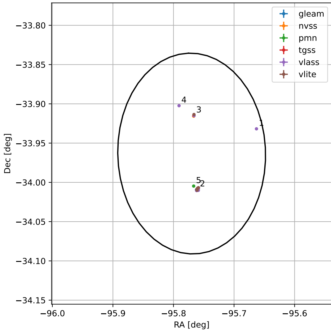
4FGL J1736.9-3357
