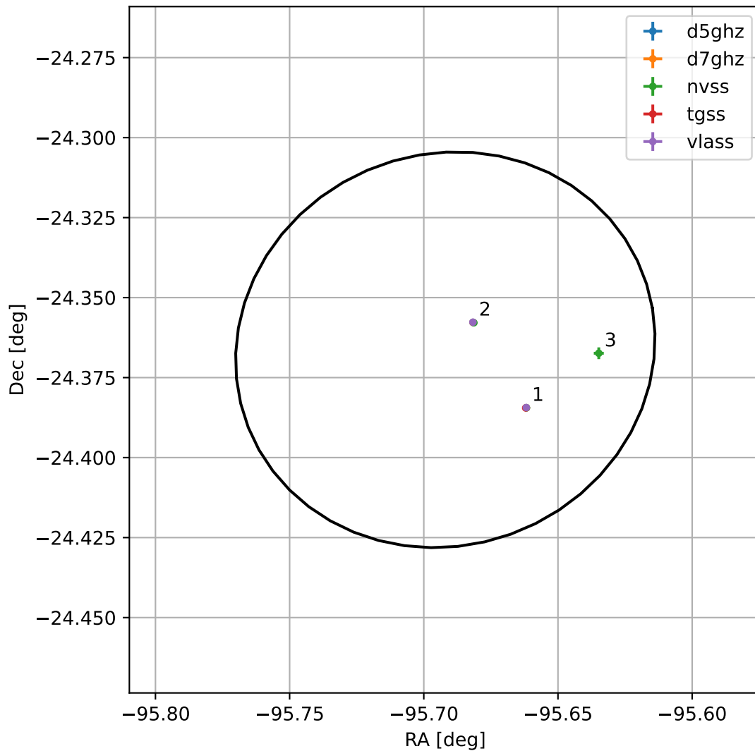
4FGL J1737.2-2421
