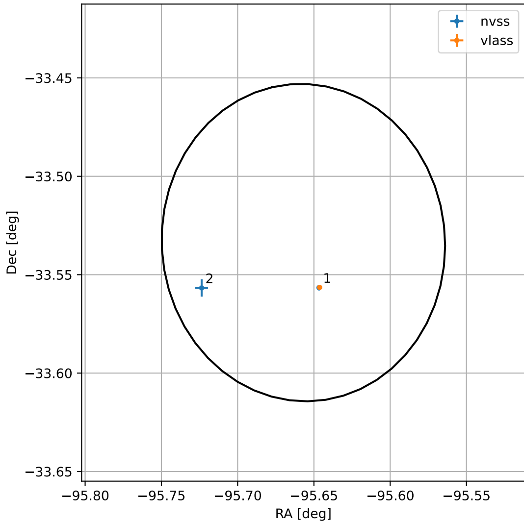
4FGL J1737.3-3332
