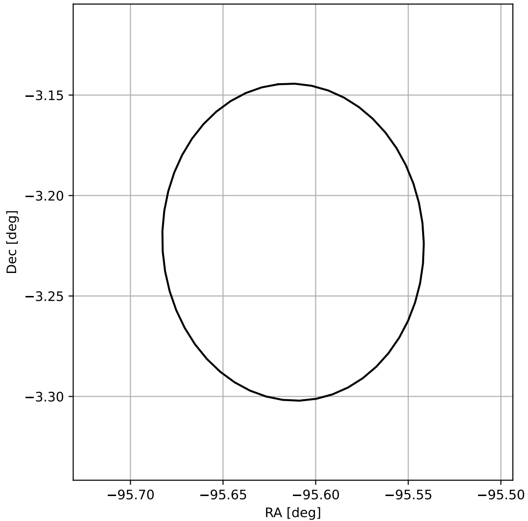
4FGL J1737.5-0313
