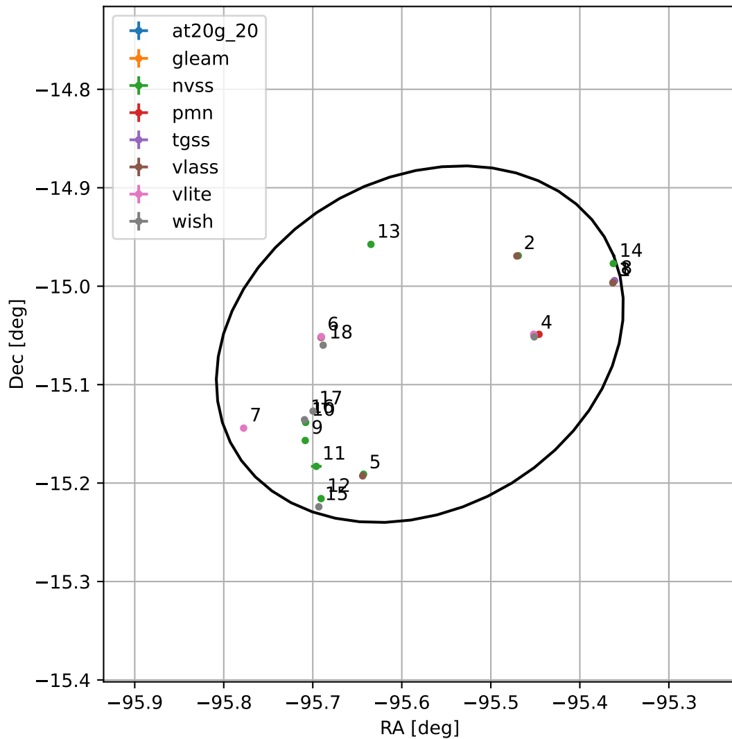
4FGL J1737.6-1503
