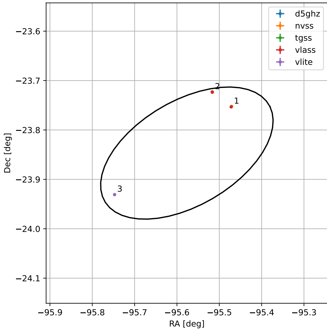
4FGL J1737.6-2350
