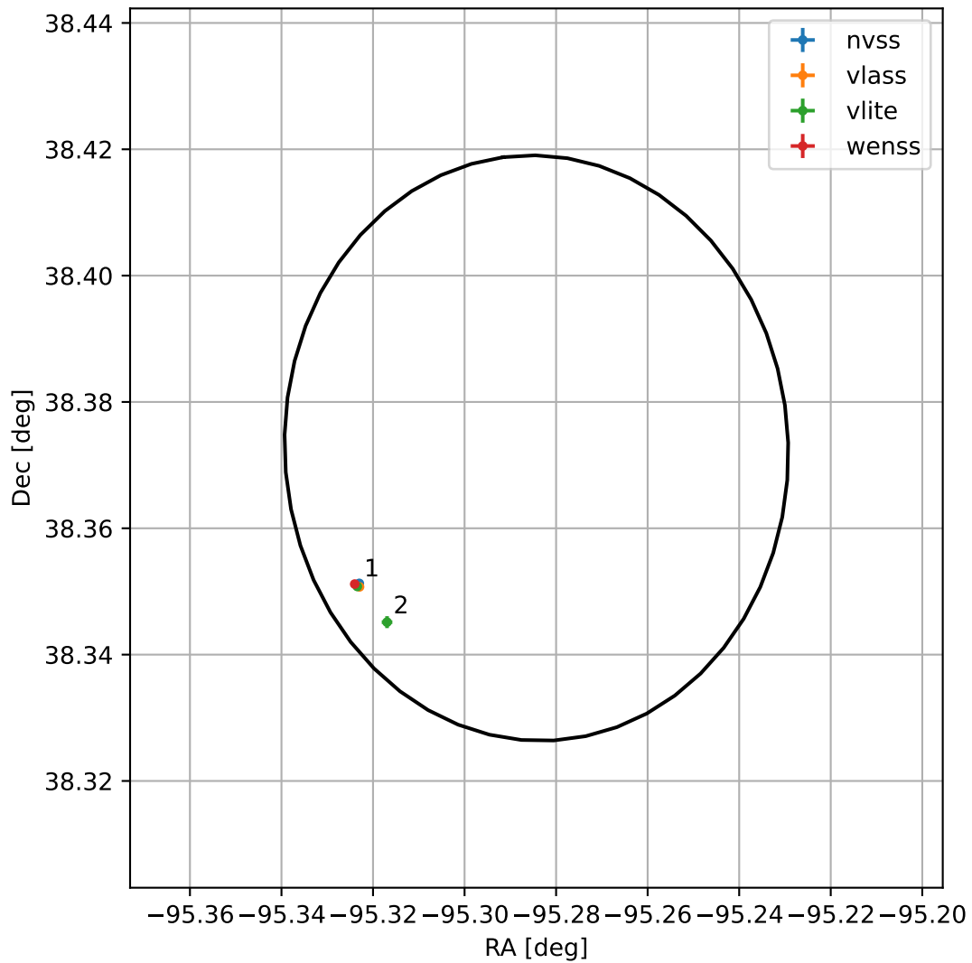
4FGL J1738.8+3822
