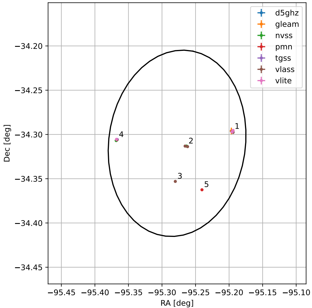
4FGL J1738.8-3418
