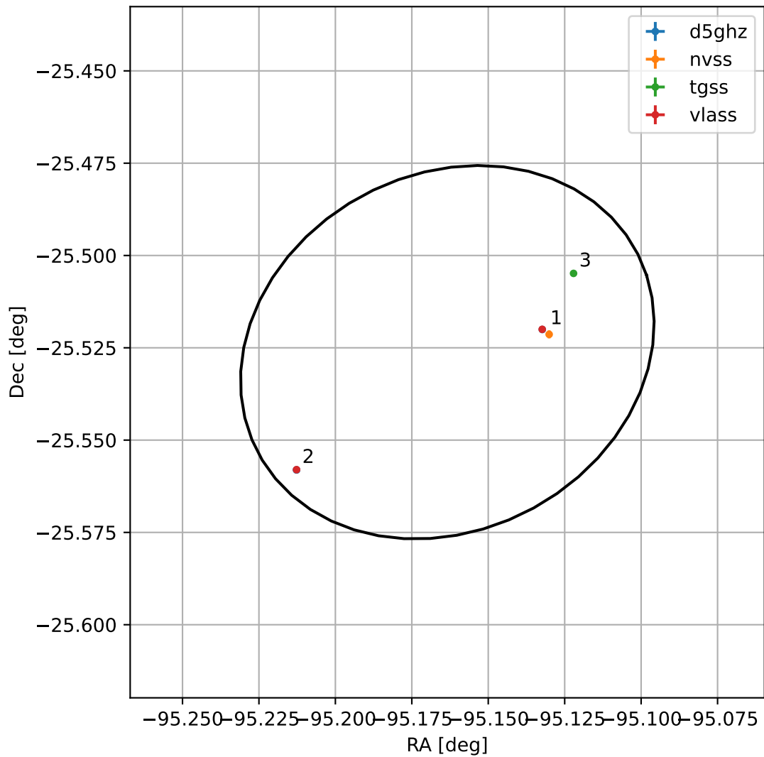
4FGL J1739.3-2531
