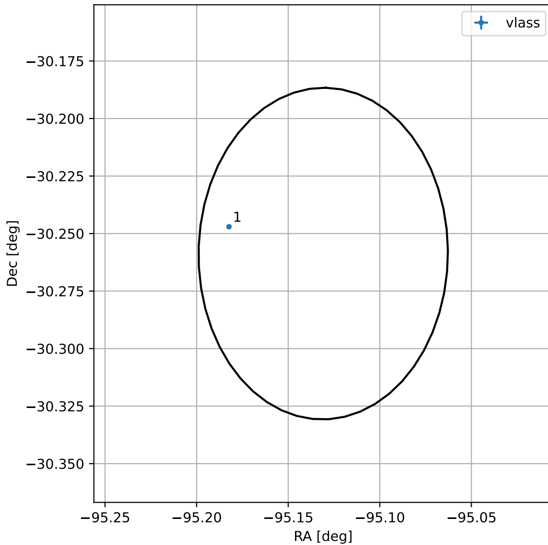
4FGL J1739.4-3015
