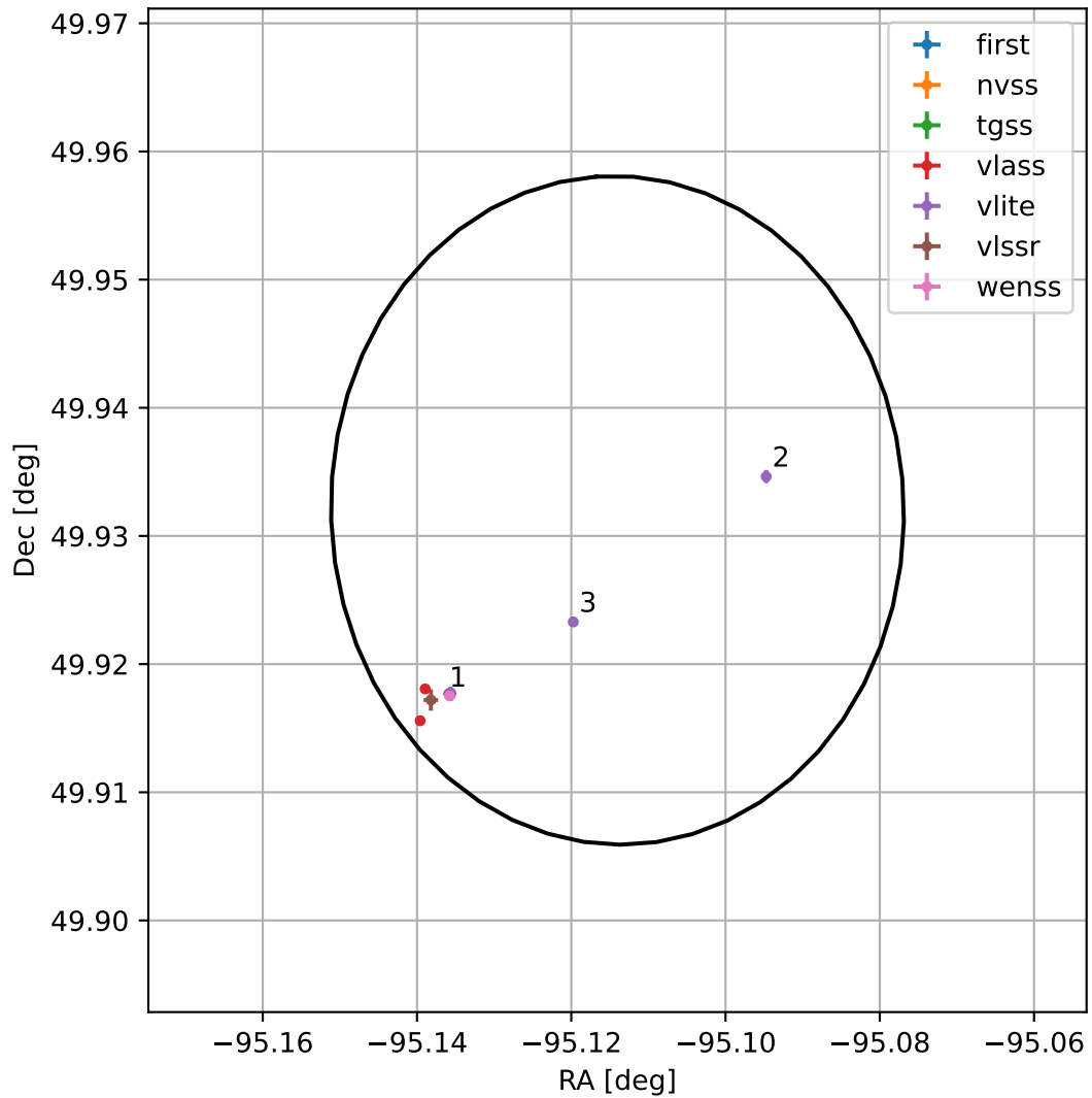
4FGL J1739.5+4955
