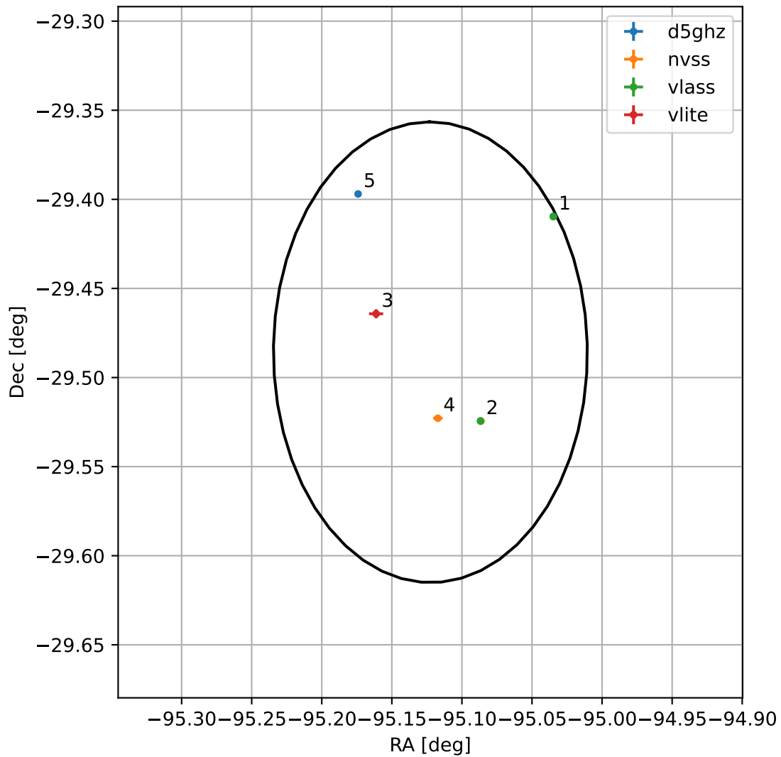
4FGL J1739.5-2929
