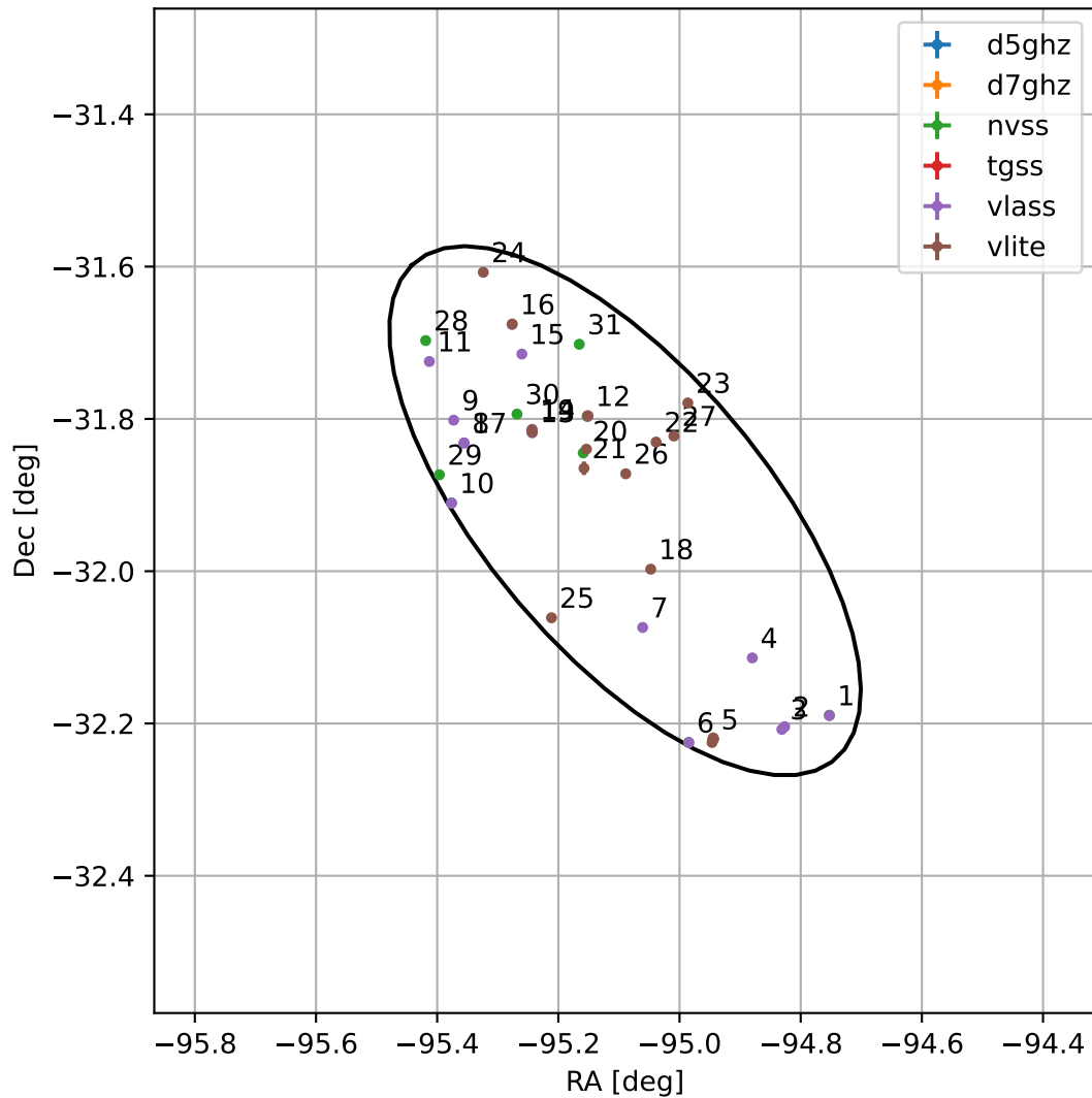
4FGL J1739.6-3155
