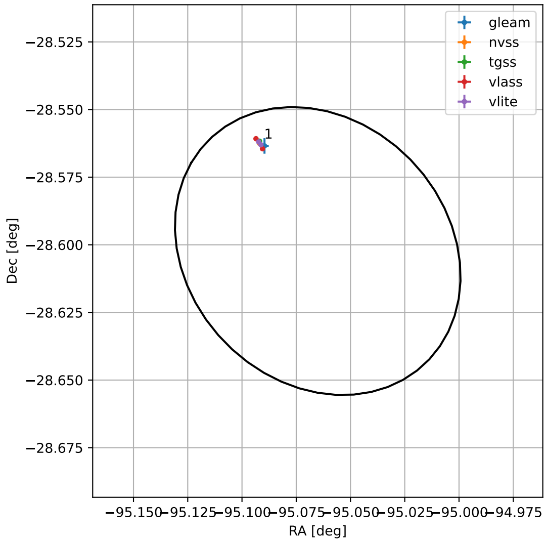
4FGL J1739.7-2836
