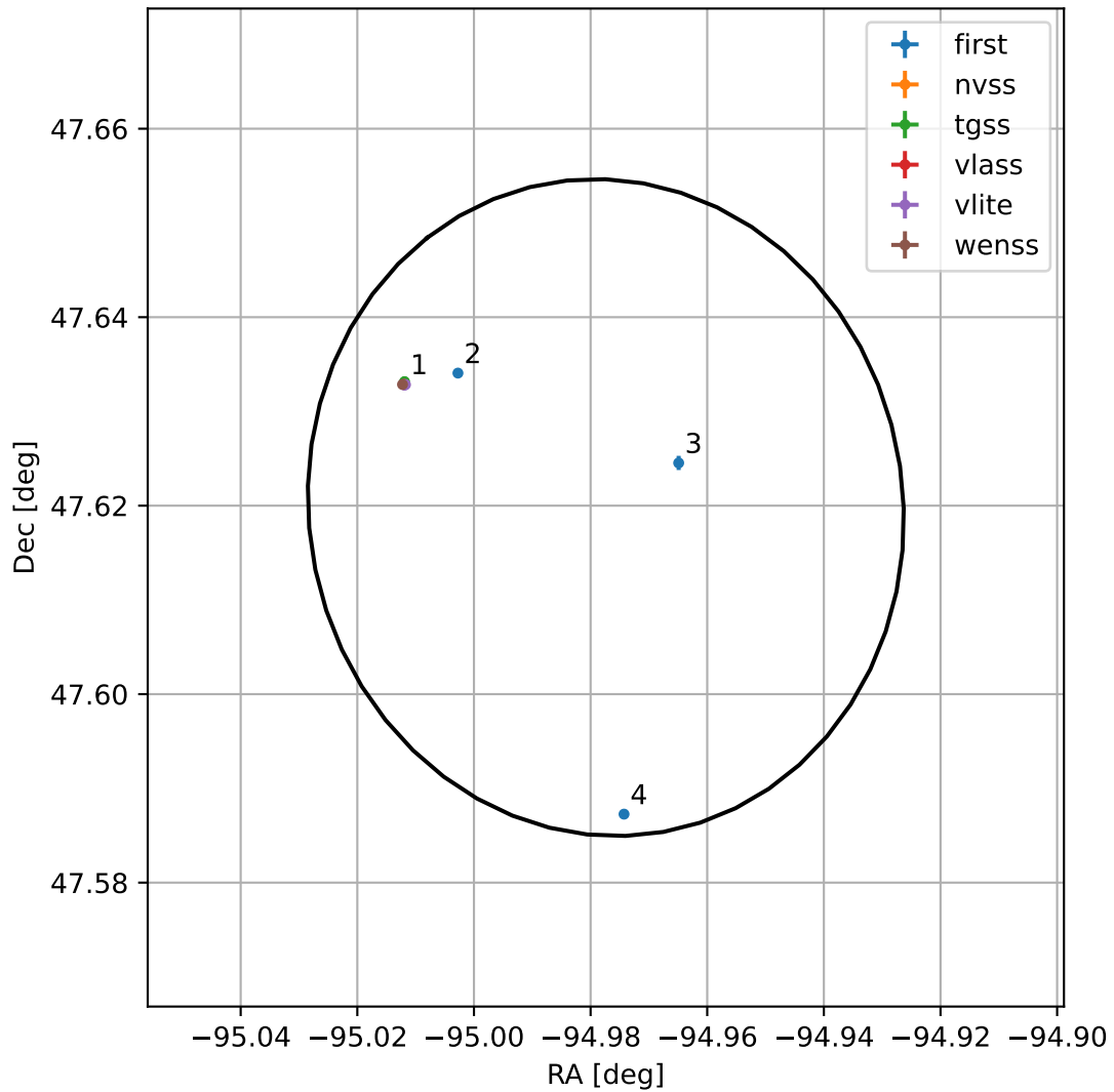
4FGL J1740.0+4737
