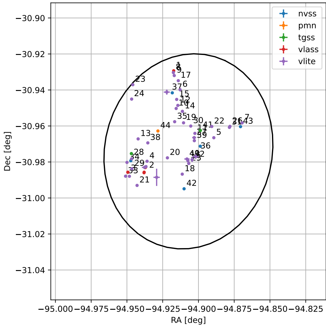
4FGL J1740.3-3058
