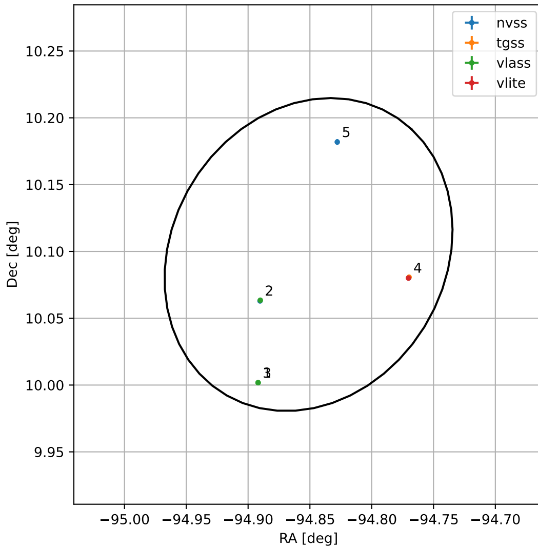
4FGL J1740.5+1005
