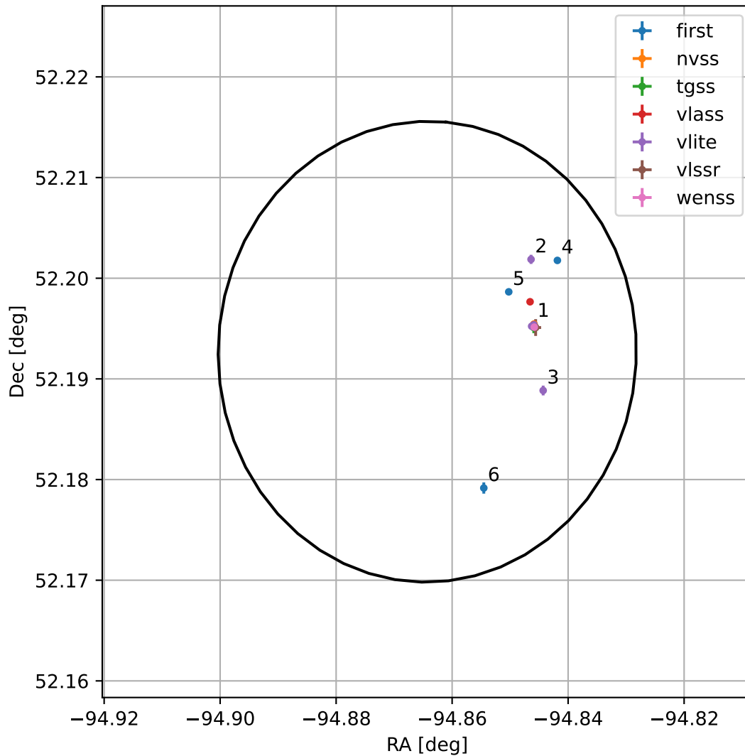
4FGL J1740.5+5211
