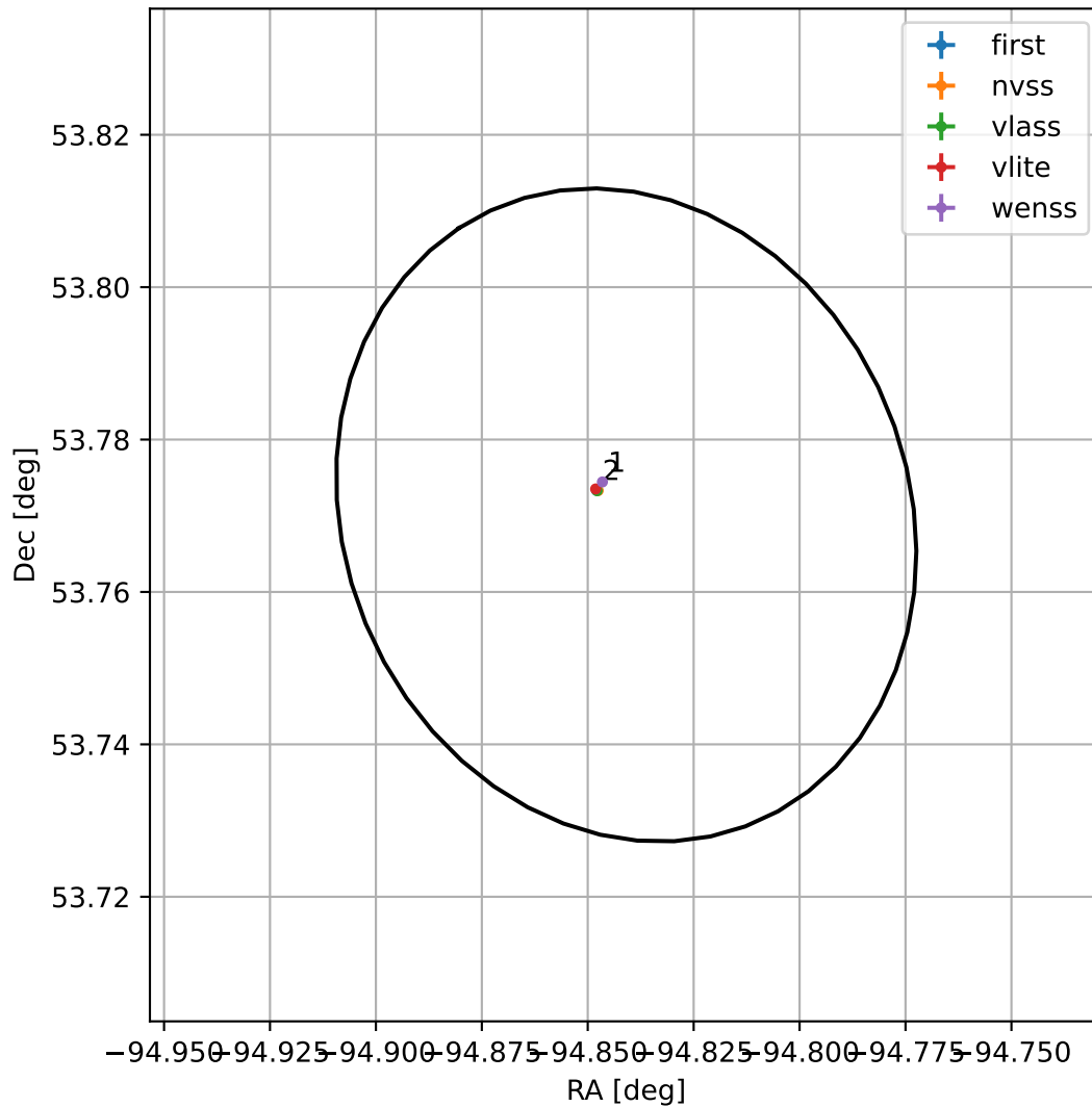
4FGL J1740.6+5346
