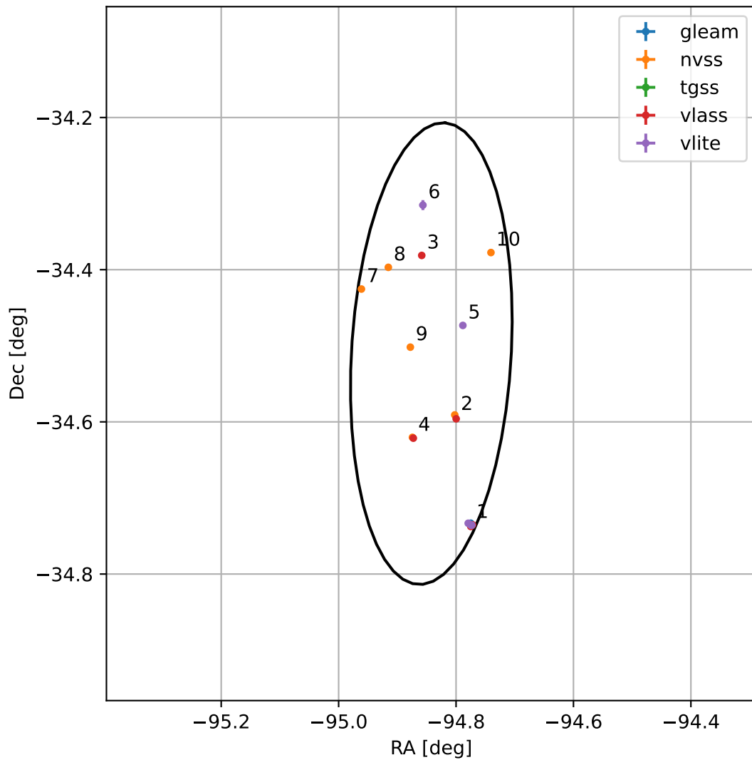
4FGL J1740.6-3430
