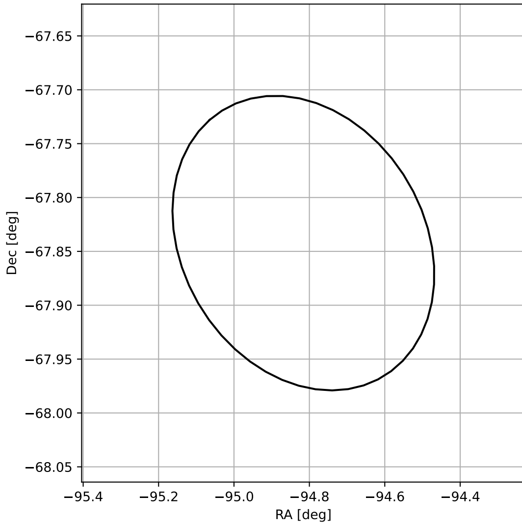
4FGL J1740.7-6750
