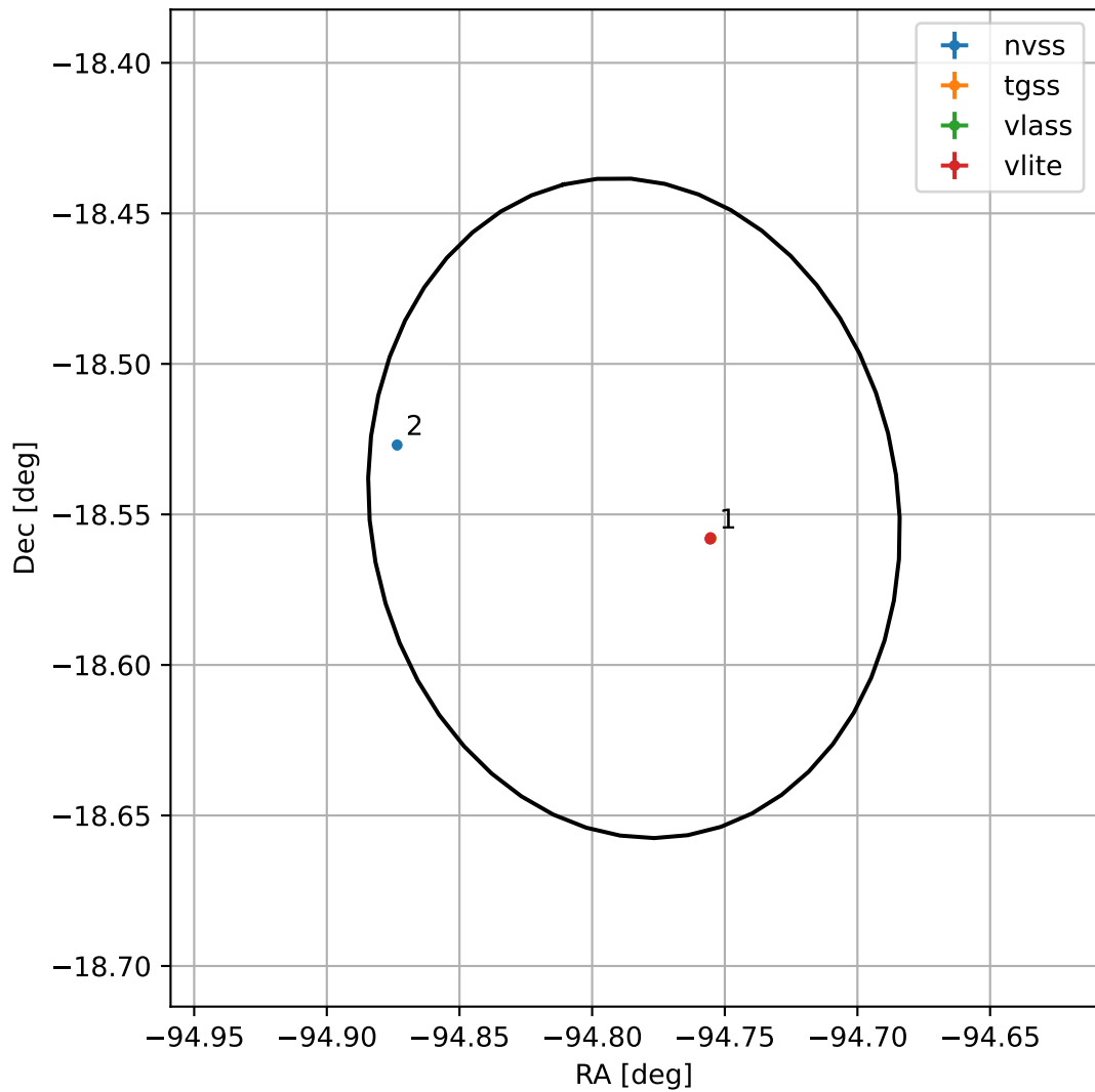
4FGL J1740.8-1832
