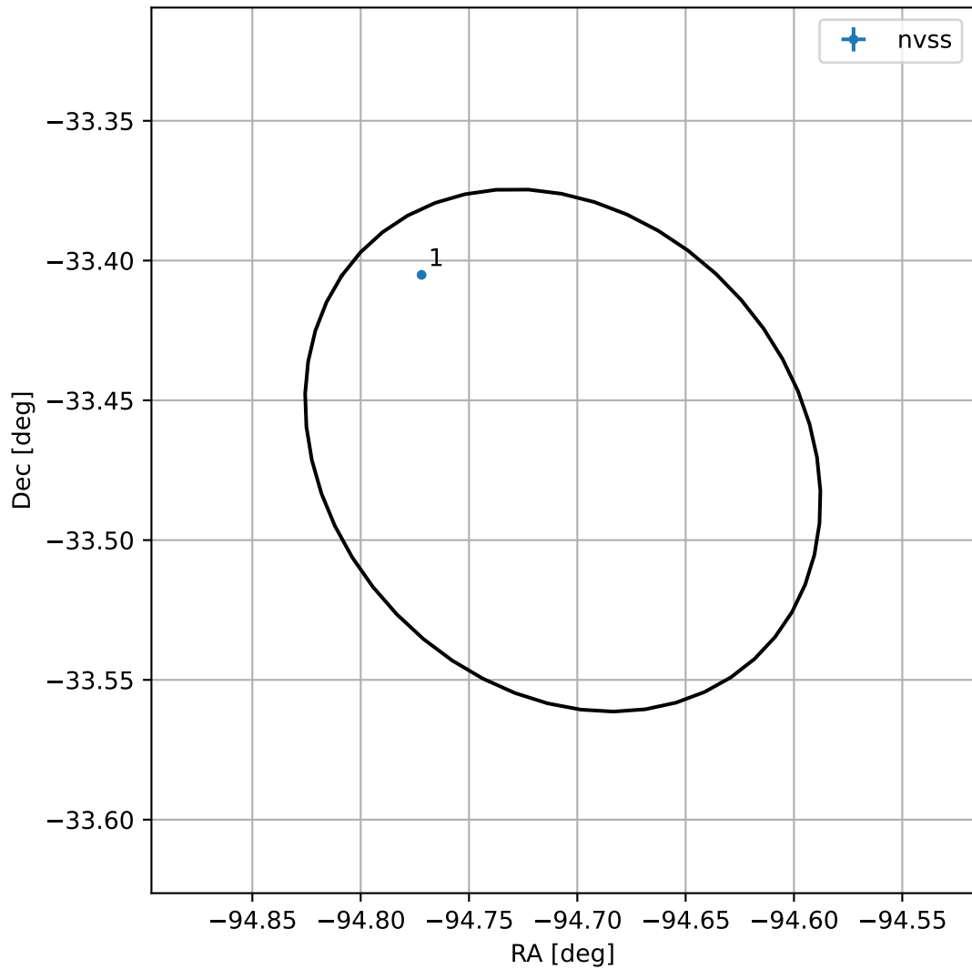
4FGL J1741.1-3328
