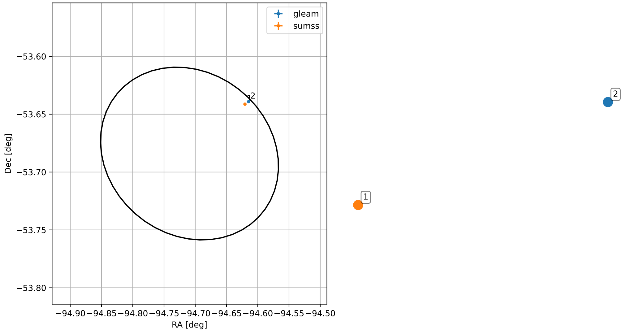
4FGL J1741.1-5341
