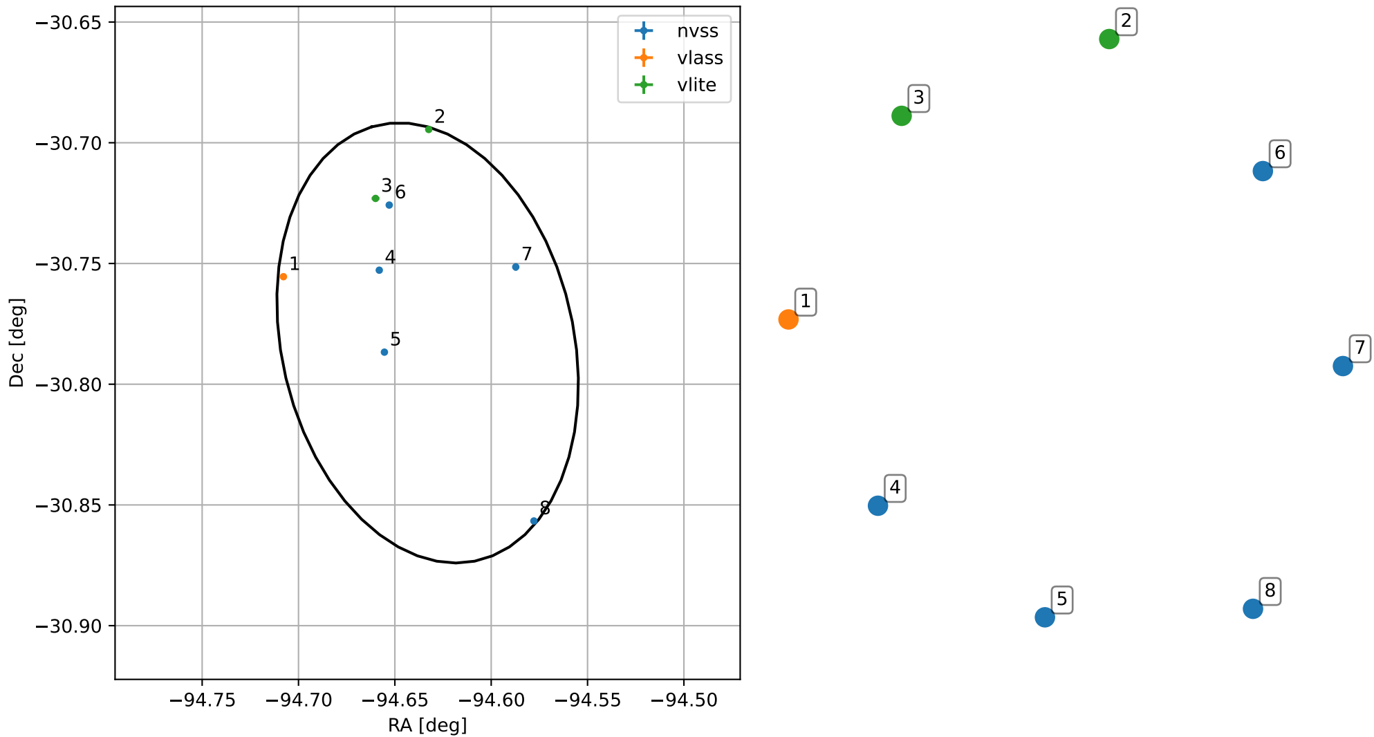
4FGL J1741.4-3046
