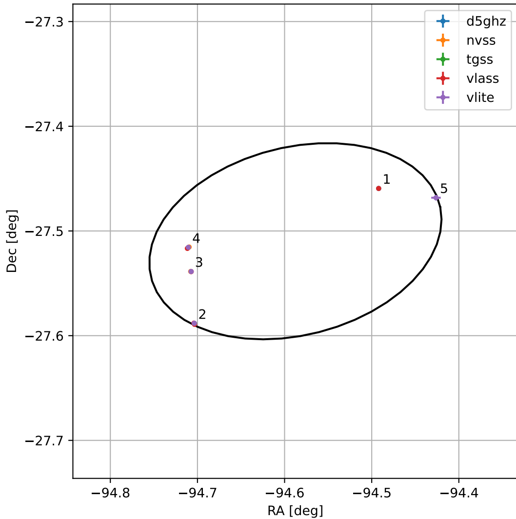
4FGL J1741.6-2730
