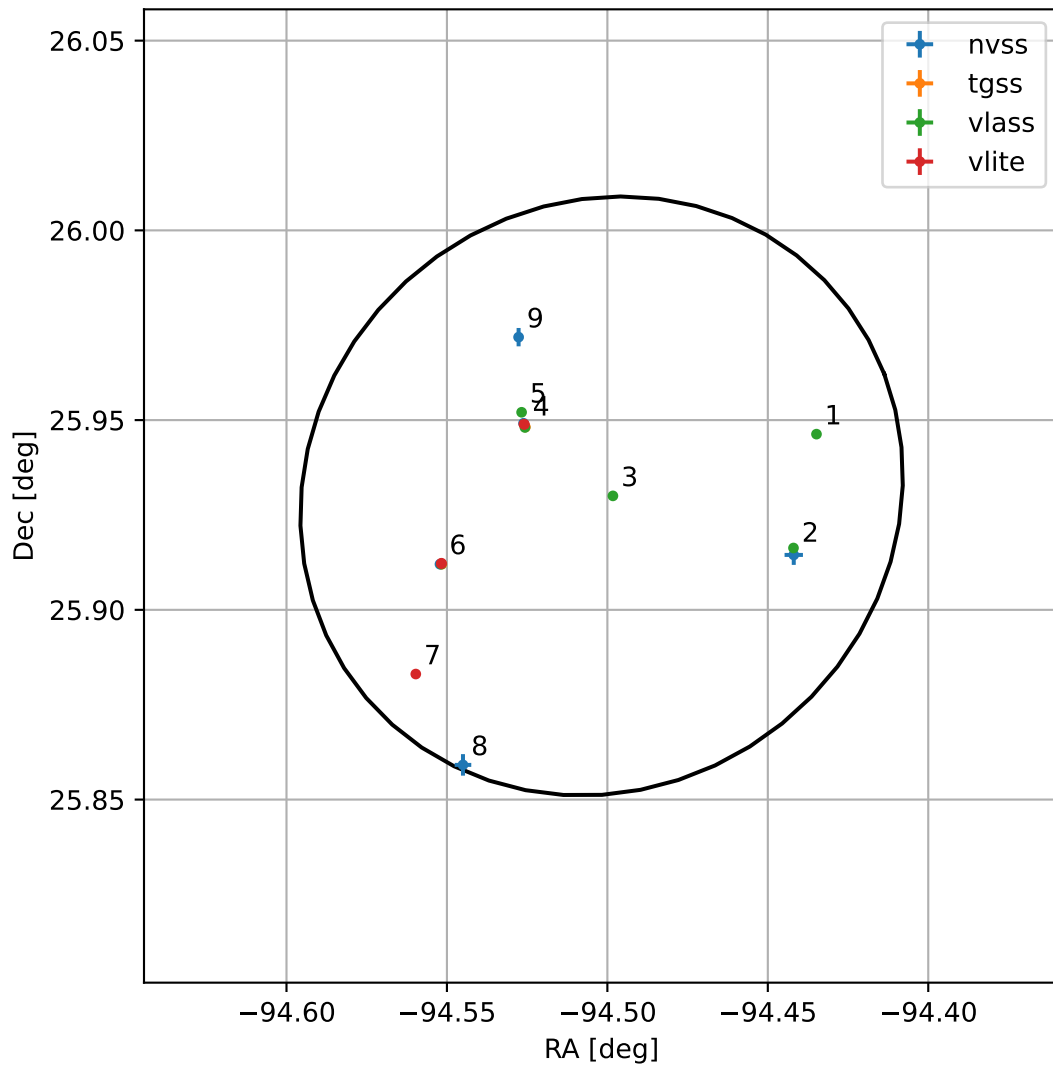
4FGL J1741.9+2555
