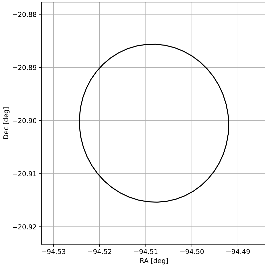
4FGL J1741.9-2054
