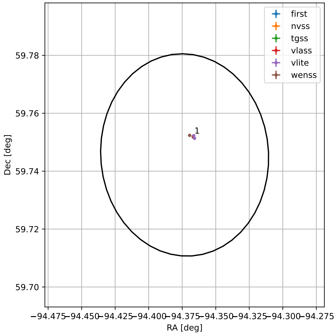
4FGL J1742.5+5944
