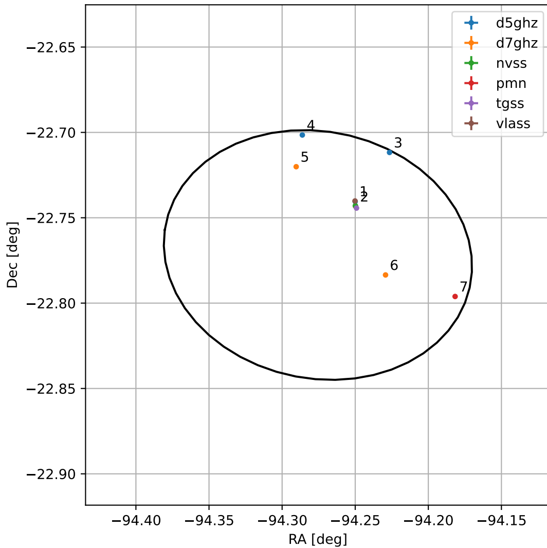
4FGL J1742.8-2246
