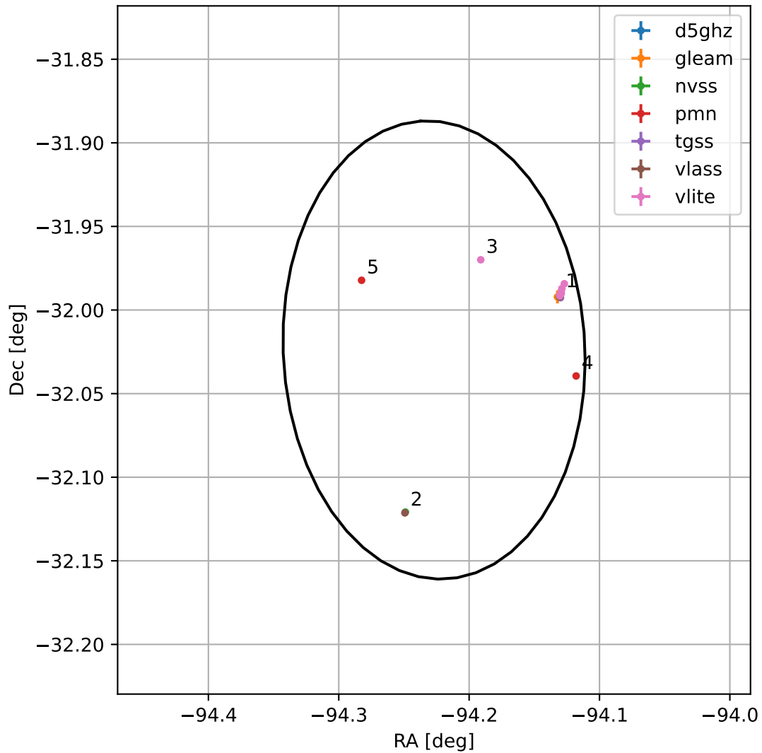
4FGL J1743.0-3201
