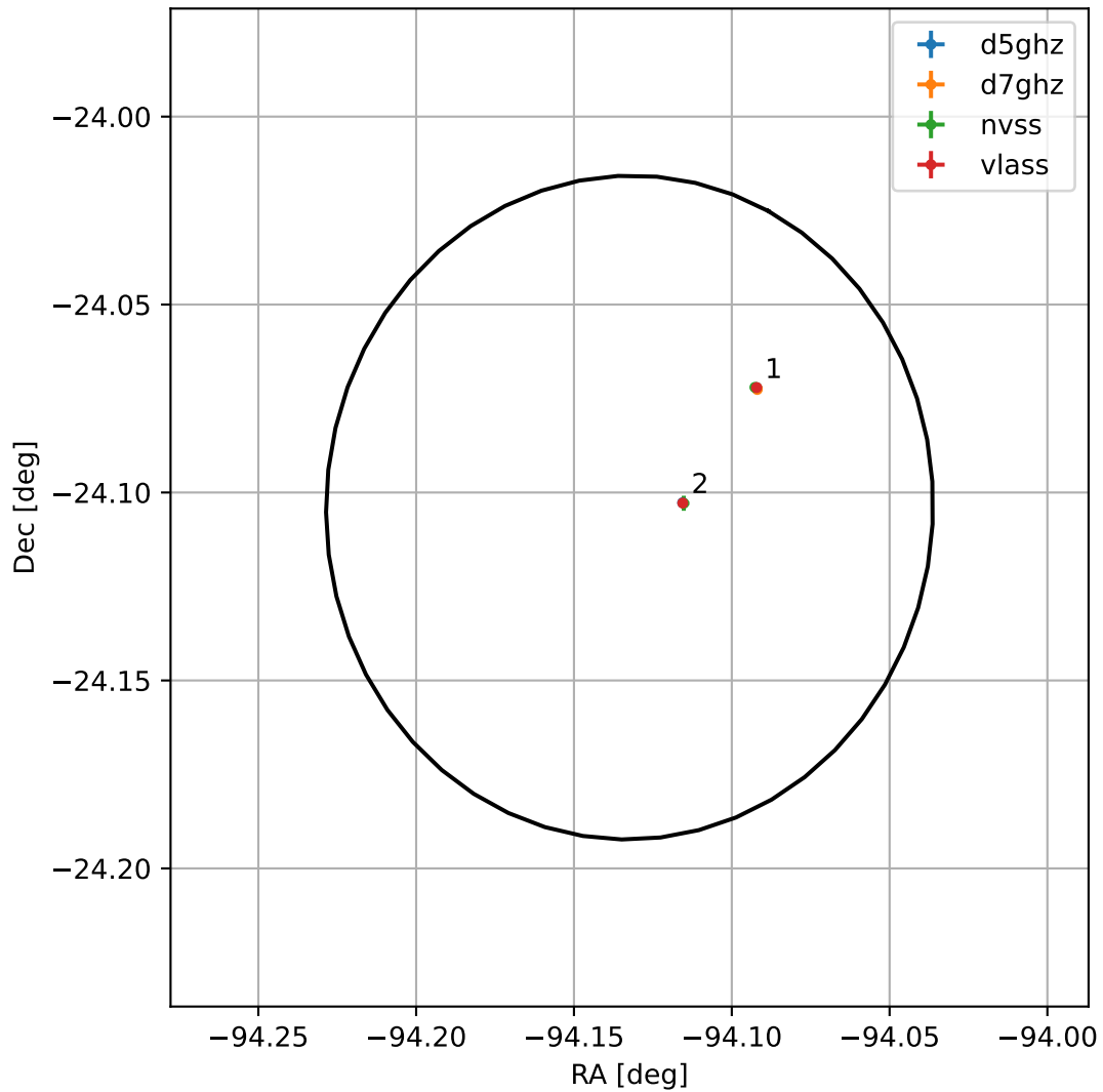
4FGL J1743.4-2406
