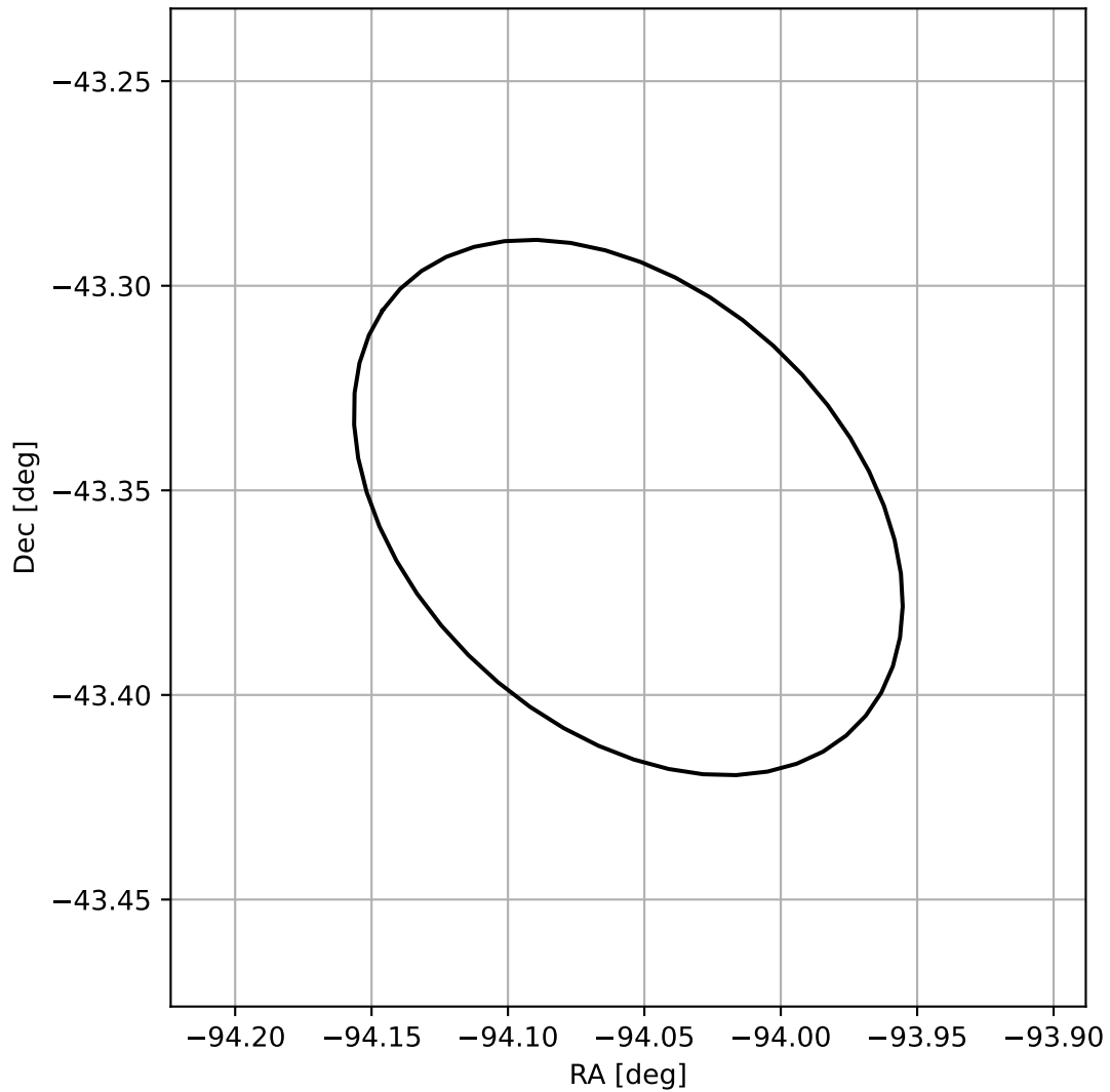
4FGL J1743.7-4321
