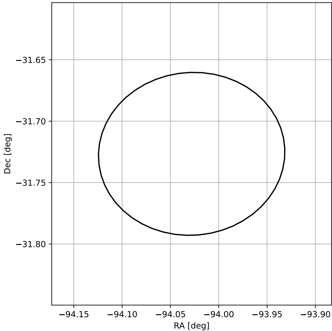
4FGL J1743.8-3143
