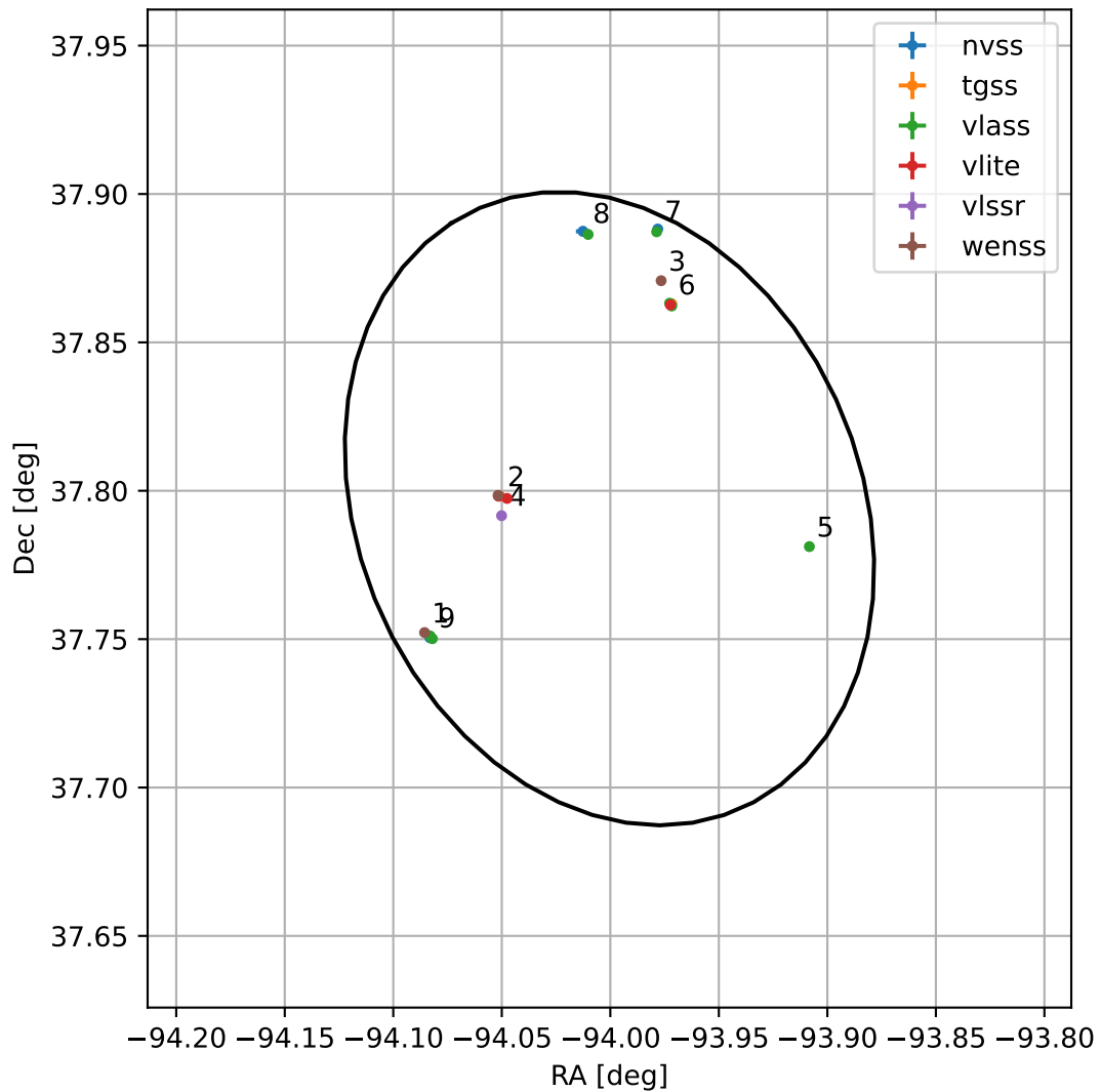
4FGL J1743.9+3747
