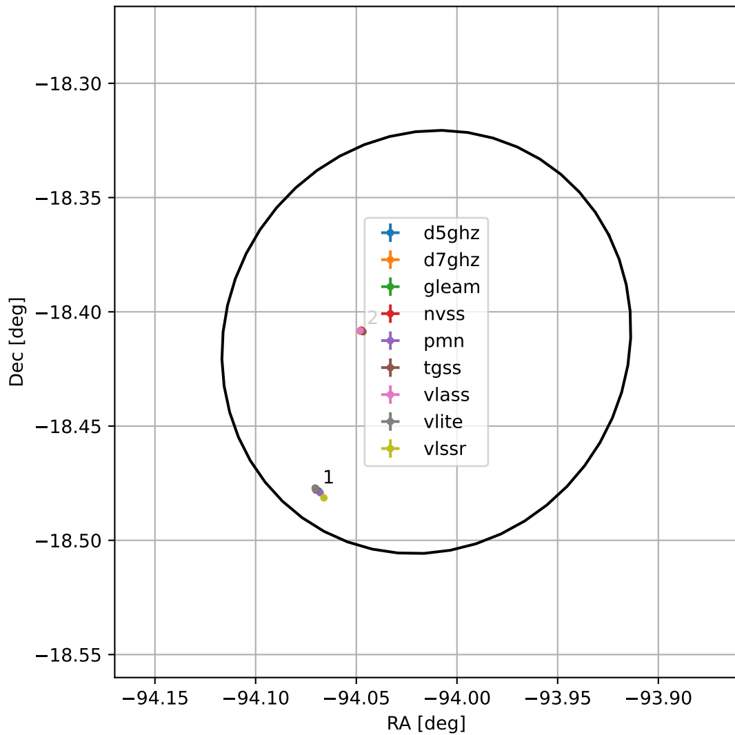
4FGL J1743.9-1824
