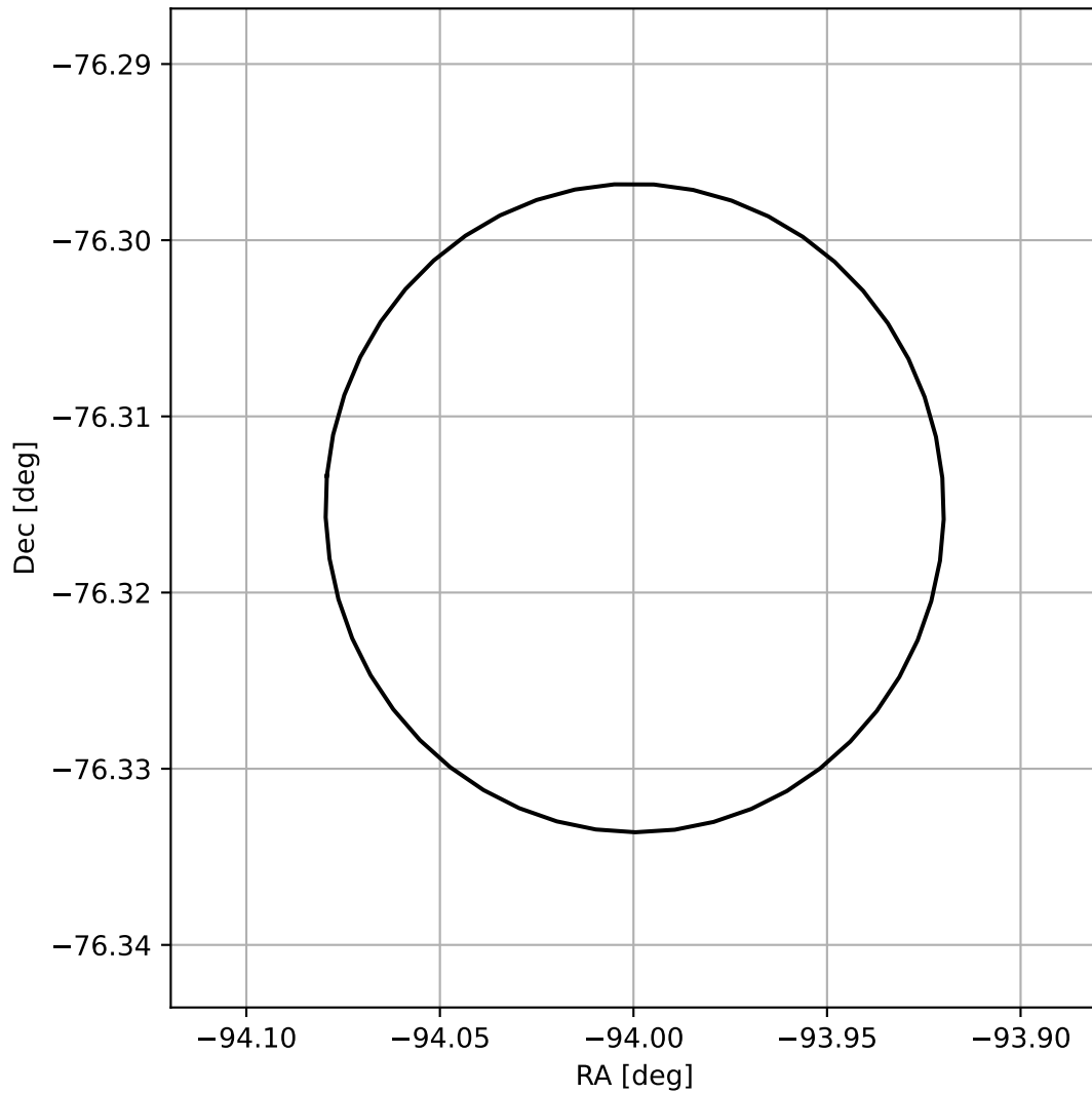
4FGL J1744.0-7618
