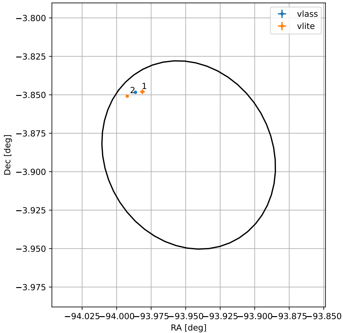
4FGL J1744.2-0353
