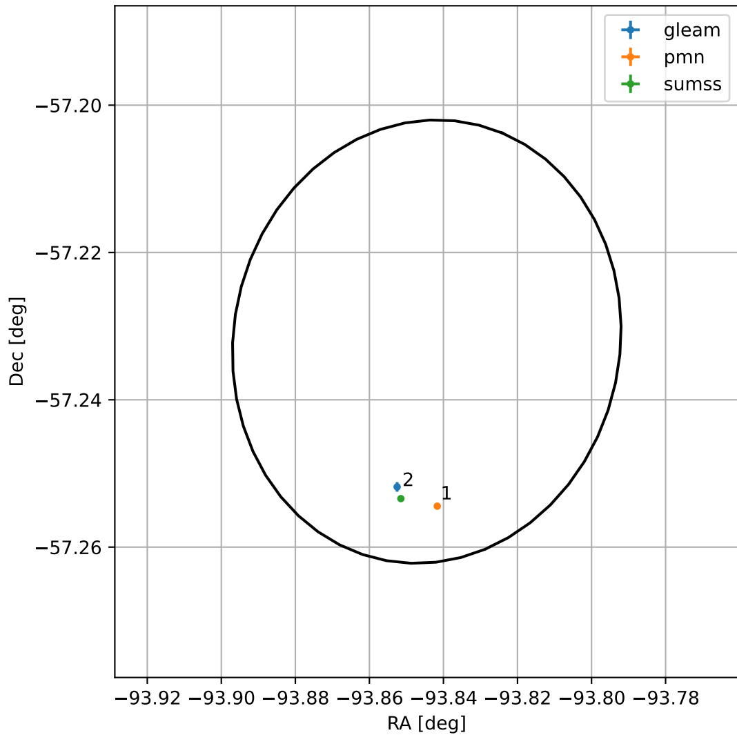
4FGL J1744.6-5713
