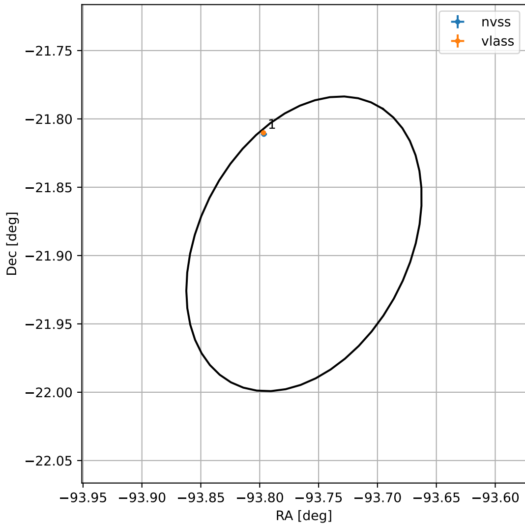
4FGL J1744.9-2153
