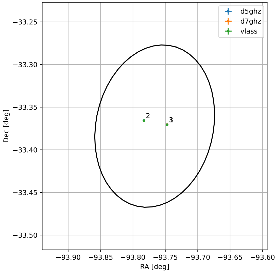
4FGL J1744.9-3322
