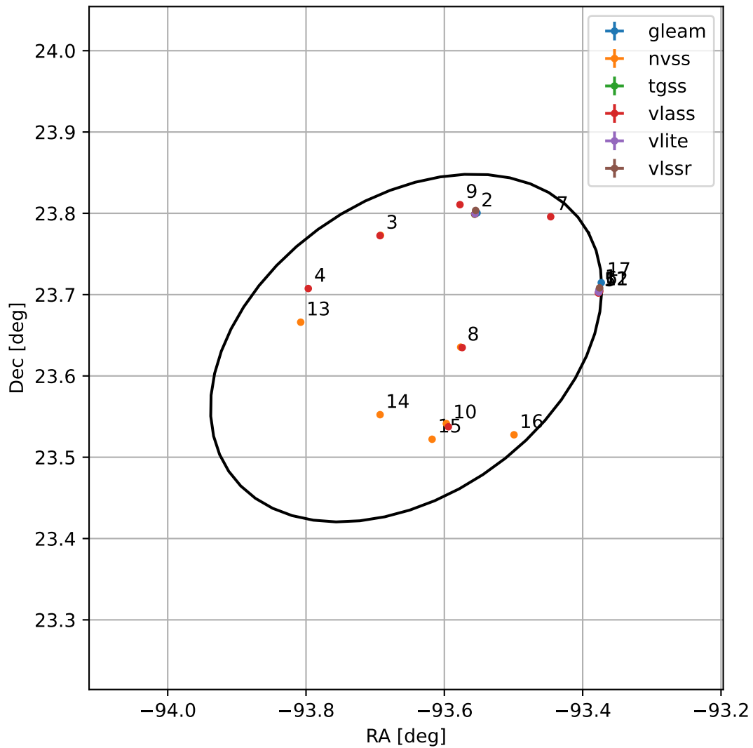
4FGL J1745.3+2338
