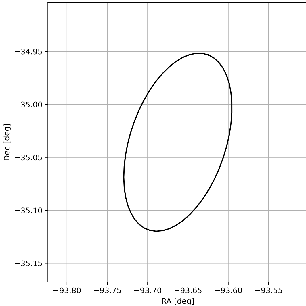
4FGL J1745.3-3502
