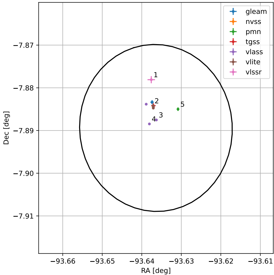
4FGL J1745.4-0753
