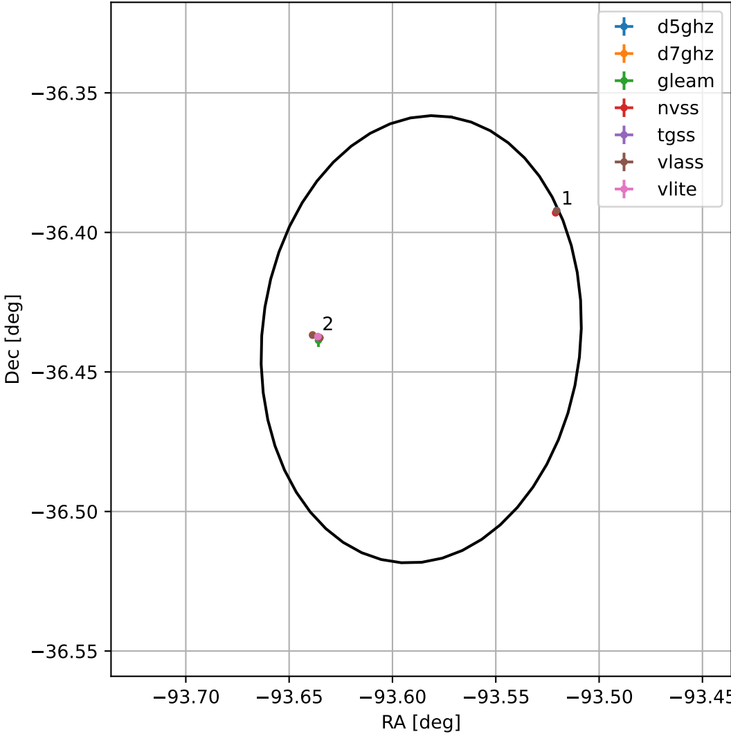
4FGL J1745.6-3626
