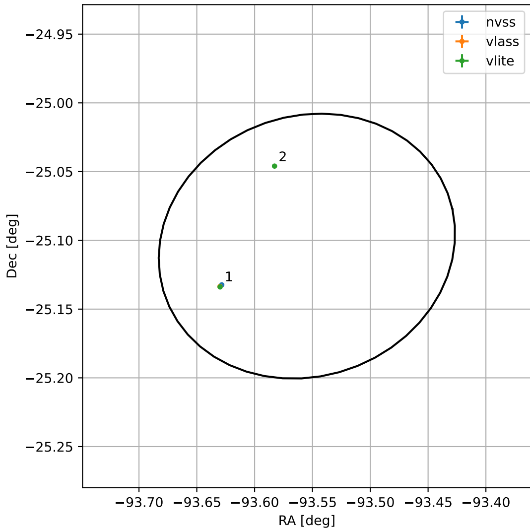
4FGL J1745.7-2506
