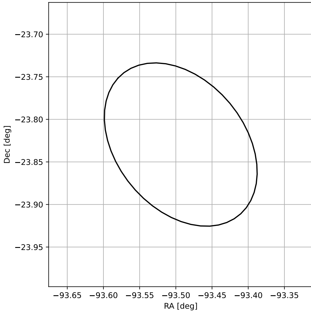
4FGL J1746.0-2349
