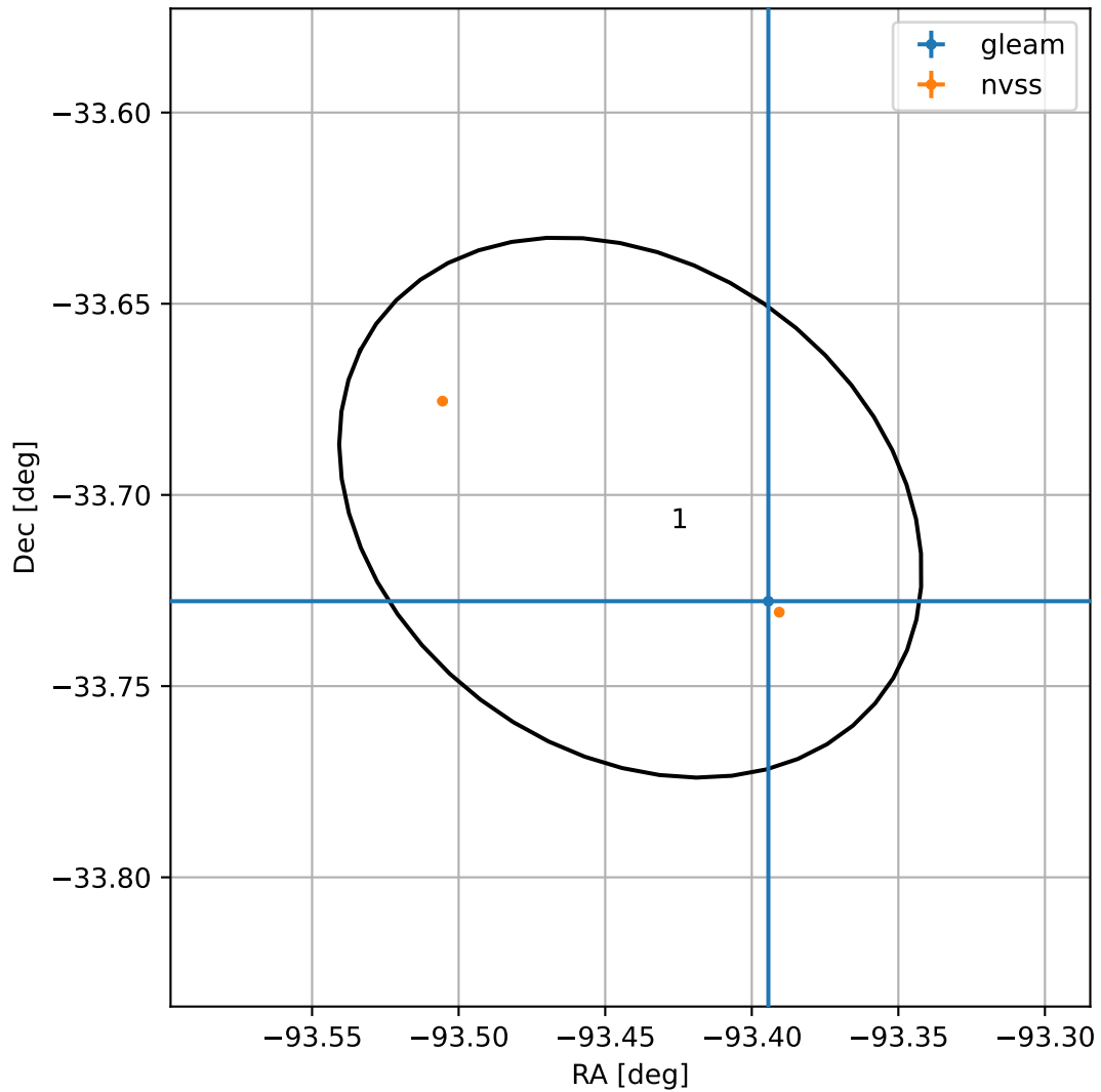
4FGL J1746.2-3342
