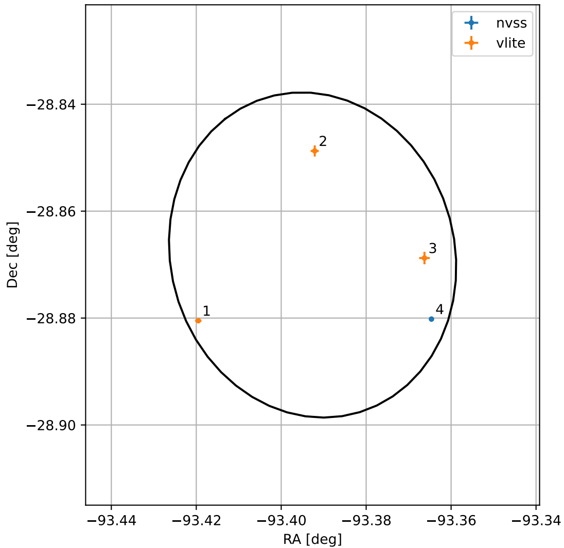
4FGL J1746.4-2852
